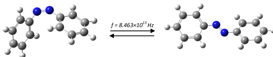
Figure 4. Photochromism of azobenzene under the radiation of frequency f = 8.463 \times 10^{13} Hz. Blue spheres represent nitrogen atoms, grey sphere represent carbon atoms and white spheres represent hydrogen atoms.
