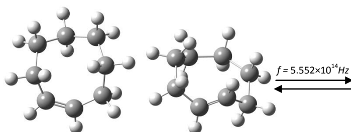
Figure 8. Photochromism of cyclooctane under the radiation of frequency f = 5.552 \times 10^{14} \text{ Hz} . Grey sphere represent carbon atoms and white spheres represent hydrogen atoms.
