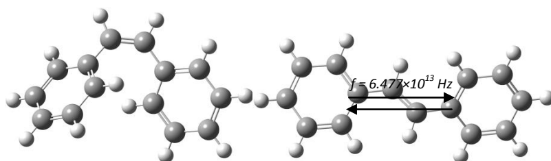
Figure 12. Photochromism of stilbene under the radiation of frequency f = 6.477 \times 10^{13} \text{ Hz} . Grey sphere represent carbon atoms and white spheres represent hydrogen atoms.
