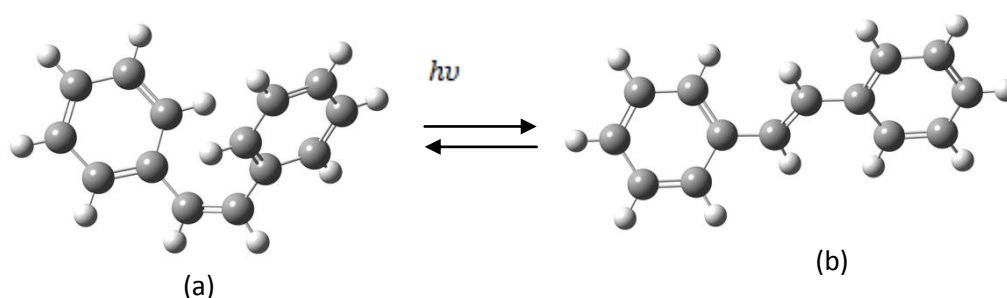
Figure 1: Photochromism in Stilbene molecule. (a) cis-stilbene (b) trans-stilbene. Grey spheres represent hydrogen atoms and black spheres represent carbon atoms.
