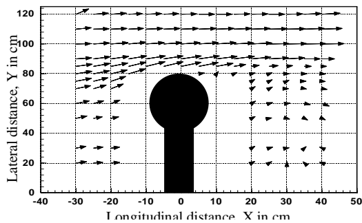
Fig. 25. Velocity vector at 0.6 depths for 170-S-90
