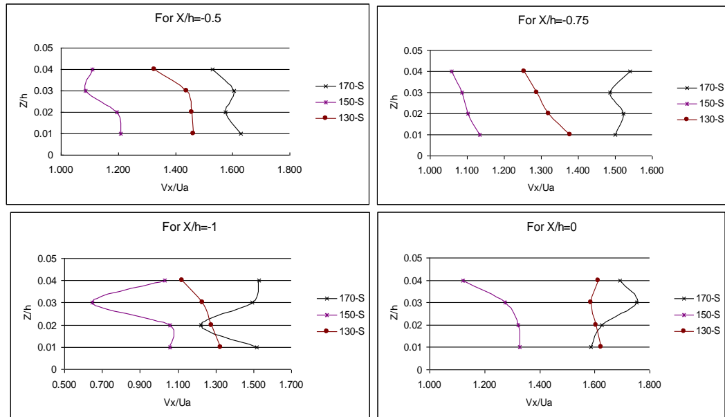
Fig. 14. Vertical variation of streamwise velocity ( V_x ) at Y/h=4.25 for 90 degree angle.
