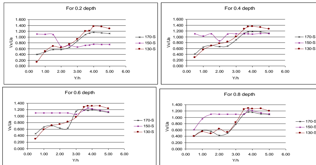
Fig. 9. Variation of streamwise velocity ( V_x ) at X/h=-5.5 in lateral direction ( Y ) for 150 degree angle
