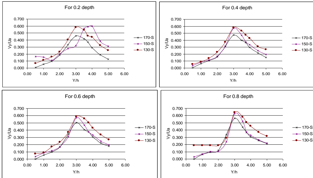
Fig. 11. Variation of transverse velocity ( V_y ) at X/h=-5.5 in lateral direction ( Y ) for 150 degree angle
