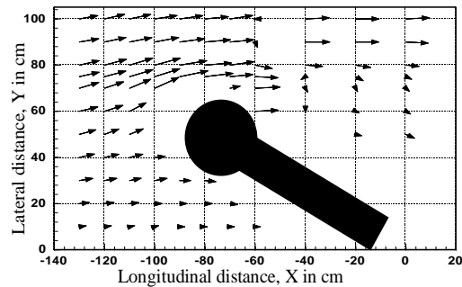
Fig. 32. Velocity vector at 0.4 depths for 130-S-150
