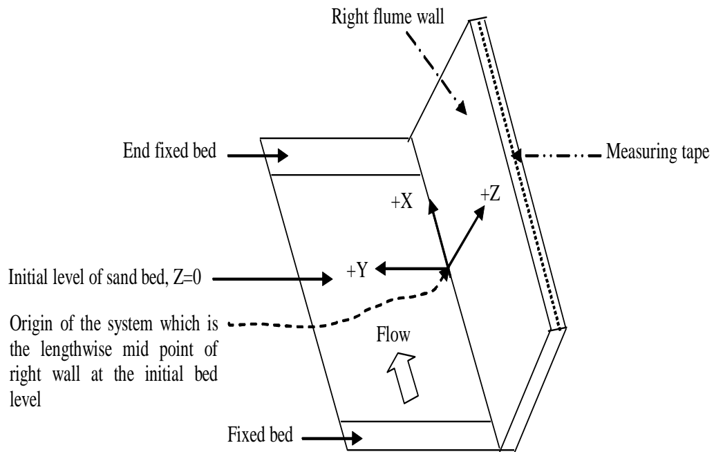
Fig. 3. Coordinate system used in the experiment
