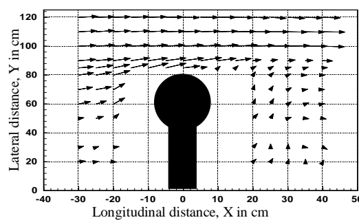
Fig. 26. Velocity vector at 0.8 depths for 170-S-90
