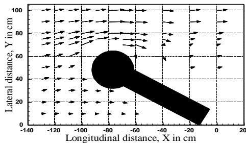
Fig. 17. Velocity vector at 0.6 depths for 170-S-150
