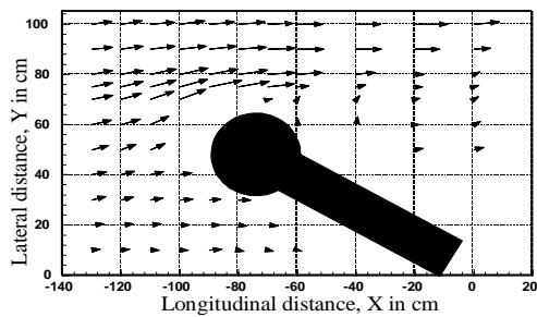
Fig. 15. Velocity vector at 0.2 depths for 170-S-150
