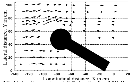
Fig.19. Velocity vector at 0.2 depths for 150-S-150
