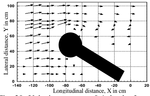
Fig. 20. Velocity vector at 0.4 depths for 150-S-150
