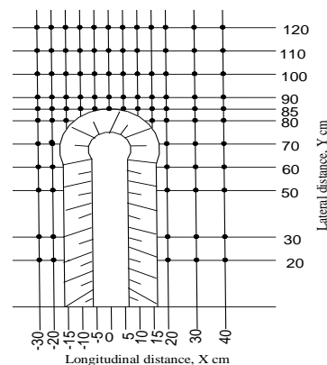
Fig. 2. Grids for velocity measurement for 90° angle
