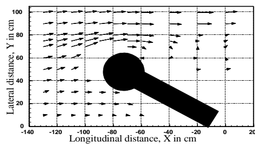
Fig. 16. Velocity vector at 0.4 depths for 170-S-150
