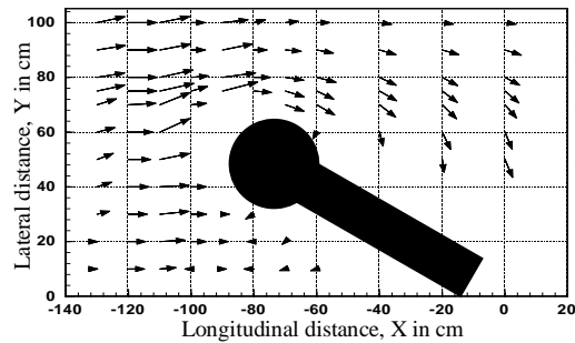
Fig. 22. Velocity vector at 0.8 depths for 150-S-150
