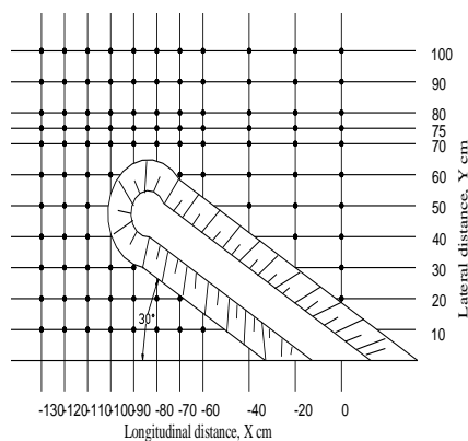
Fig. 1. Grids for velocity measurement for 150° angle
