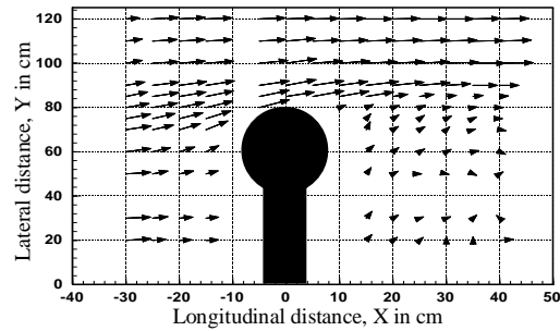
Fig. 24. Velocity vector at 0.4 depths for 170-S-90
