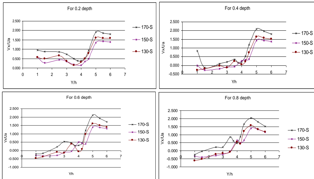
Fig. 10. Variation of streamwise velocity ( V_x ) at X/h=2 in lateral direction ( Y ) for 90 degree angle
