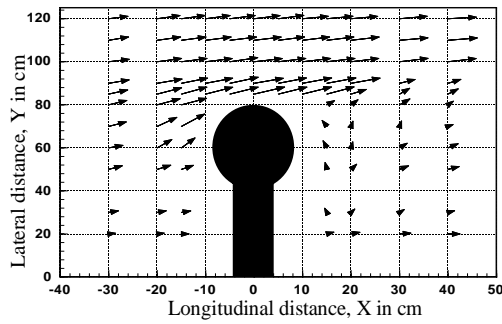
Fig. 27. Velocity vector at 0.2 depths for 150-S-90
