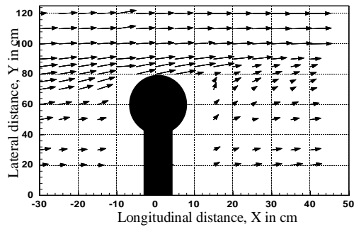
Fig. 23. Velocity vector at 0.2 depths for 170-S-90
