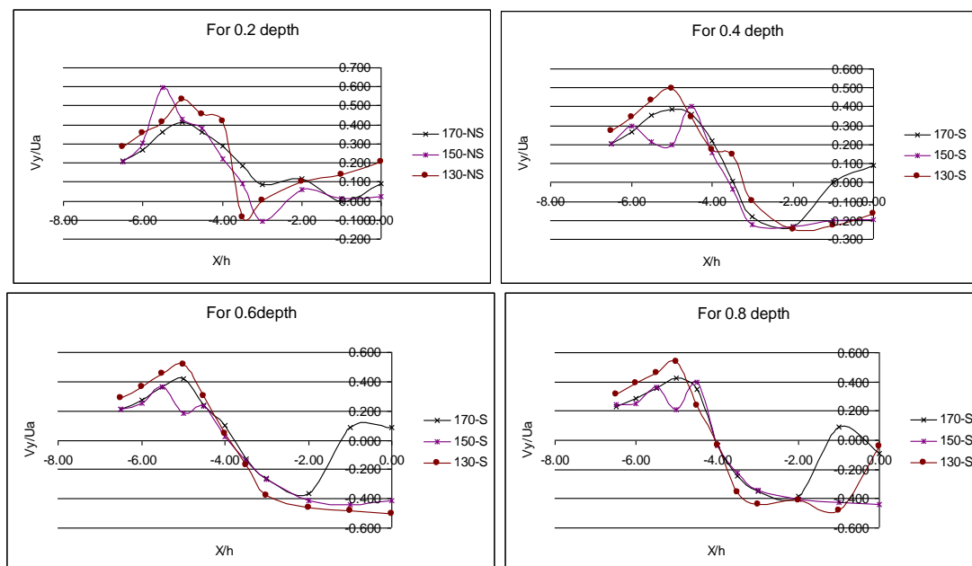
Fig. 7. Variation of transverse velocity ( V_y ) at Y/h=3.25 in longitudinal direction ( X ) for 150 degree angle
