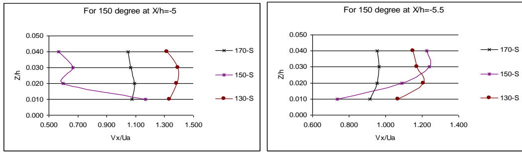
Fig. 13. Vertical variation of streamwise velocity ( V_x ) at Y/h=3.25 for 150 degree angle
