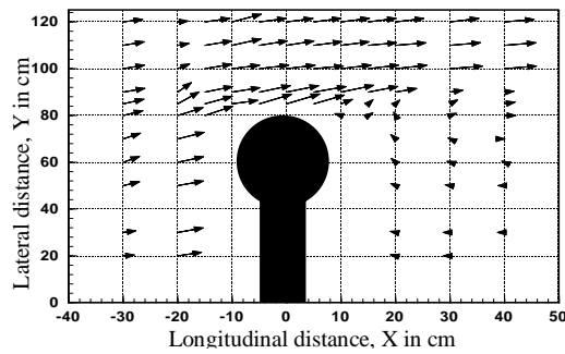
Fig. 29. Velocity vector at 0.6 depths for 150-S-90
