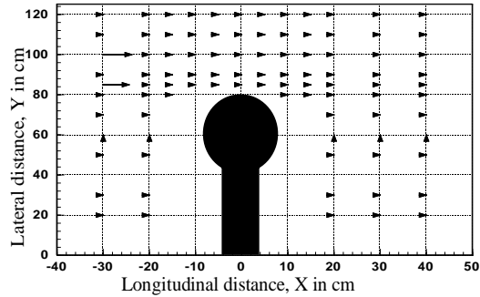
Fig. 30. Velocity vector at 0.8 depths for 150-S-90
