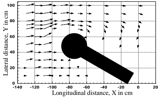
Fig. 21. Velocity vector at 0.6 depths for 150-S-150
