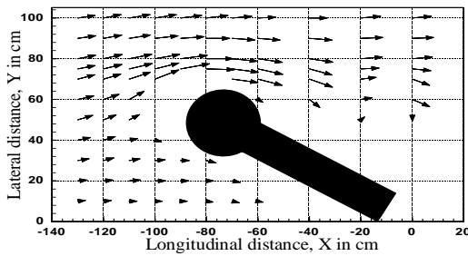
Fig. 18. Velocity vector at 0.8 depths for 170-S-150
