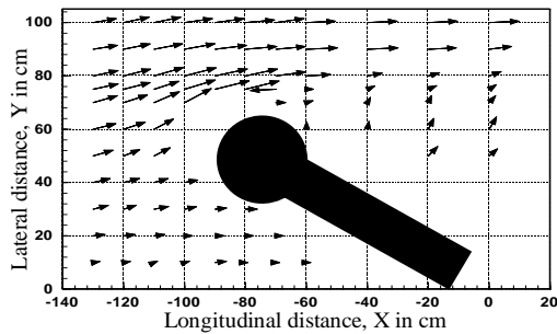
Fig. 31. Velocity vector at 0.2 depths for 130-S-150
