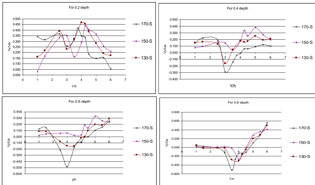
Fig. 12. Variation of transverse velocity ( V_y ) at X/h=2 in lateral direction ( Y ) for 90 degree angle
