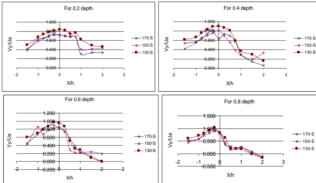
Fig. 8. Variation of transverse velocity ( V_y ) at Y/h=4.25 in longitudinal direction ( X ) for 90 degree angle
