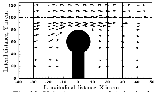
Fig. 28. Velocity vector at 0.4 depths for 150-S-90
