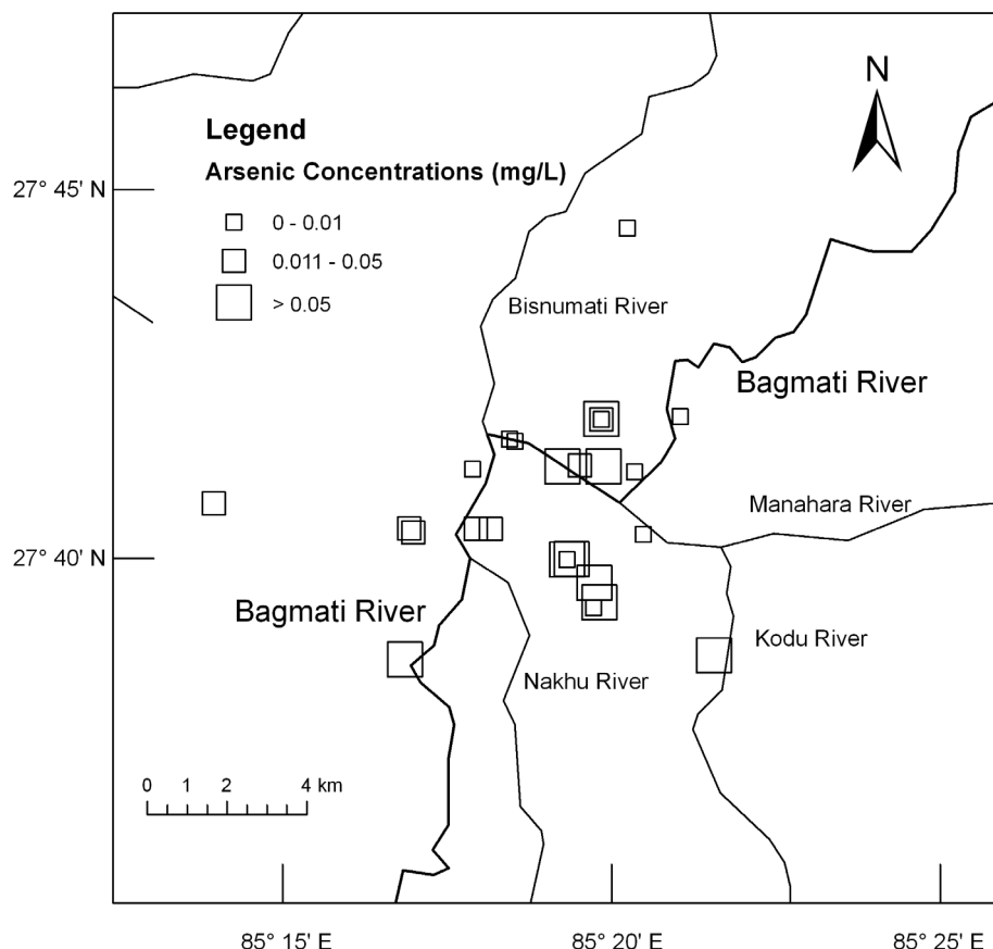
Fig. 2: Groundwater samples collected from 14 tubewells, 13 dug wells and stone spouts throughout the Kathmandu Valley (Hearn et al. 2001). Arsenic concentrations were classified as meeting the WHO As Standard ( \leq 0.01 mg/L), exceeding the WHO As Standard but meeting the Nepal Interim As Standard (0.011 – 0.05 mg/L), or exceeding the Nepal Interim As Standard ( > 0.05 mg/L).
