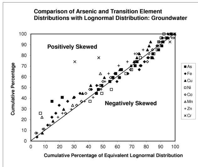
Fig. 3b: For each measured concentration of As, Fe, Cu, Ni, Co, Mn, Zn and Cr in groundwater, the percentage of measured concentrations less than or equal to that value is plotted against the percentage that would result from a lognormal distribution with the same mean and standard deviation as the set of logarithms of measured concentrations. Values below the detection limit are set equal to the detection threshold. All of the parameters follow a lognormal distribution with the exception of Cr, for which 52% of the measurements are below the detection limit.
