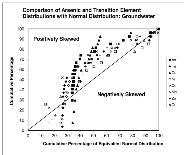
Fig. 3a: For each measured concentration of As, Fe, Cu, Ni, Co, Mn, Zn and Cr in groundwater, the percentage of measured concentrations less than or equal to that value is plotted against the percentage that would result from a normal distribution with the same mean and standard deviation as the set of measured concentrations. None of the parameters follow a normal distribution
