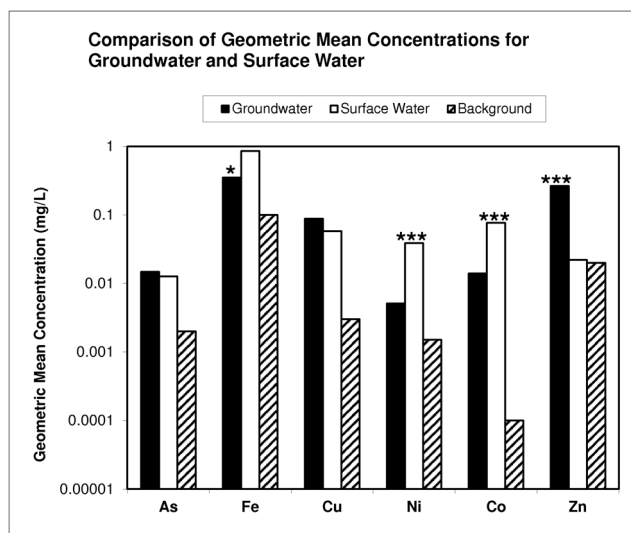
Fig. 4: The symbols *, **, *** indicate differences between geometric means of concentrations in groundwater and surface water for a given parameter are statistically significant at the 95%, 99% and 99.9% confidence levels according to the Student's t-test. Differences between concentrations of As and Cu in groundwater and surface water are not statistically significant. Concentrations of all elements are elevated in comparison with global background concentrations (Langmuir 1997) with the exception of Zn in surface water.
