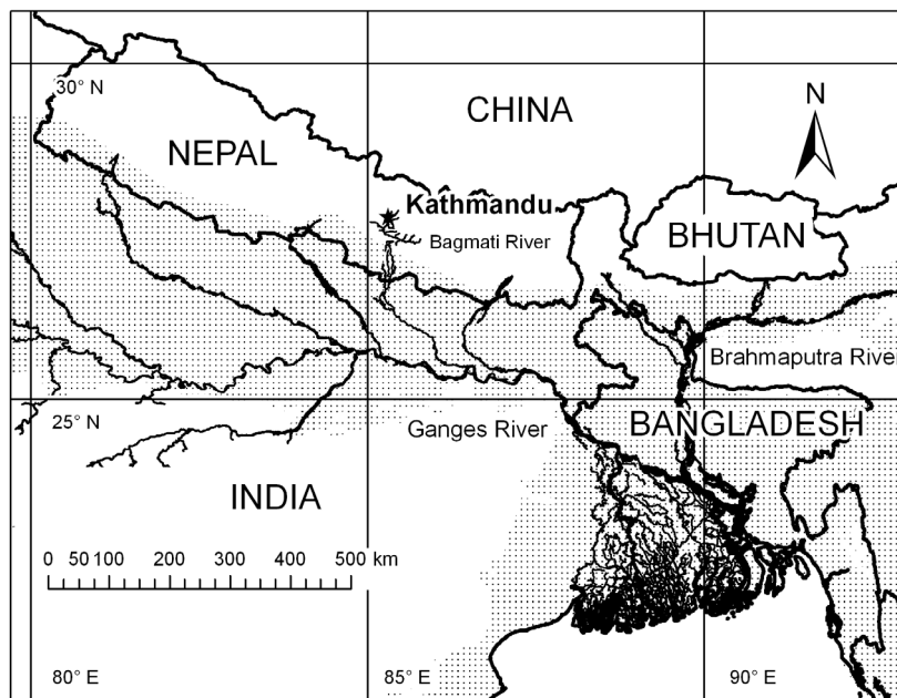
Fig. 1: The Kathmandu Valley is a heavily populated tectonic valley in the upper reaches of the Ganges River system (Hearn et al. 2001). Most of the tributaries of the Ganges River in Nepal are not shown in order to emphasize the Bagmati River
