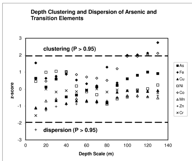
Fig. 5: Similar concentrations of both Fe and Co are clustered at depth scales \geq 100 m. No other elements, including As, show clustering at any depth scale. The z-score is calculated using the Global Moran's I-Test and the logarithms of concentrations (mg/L) in which values below the detection limit are set equal to the detection threshold (Mitchell 2005).
