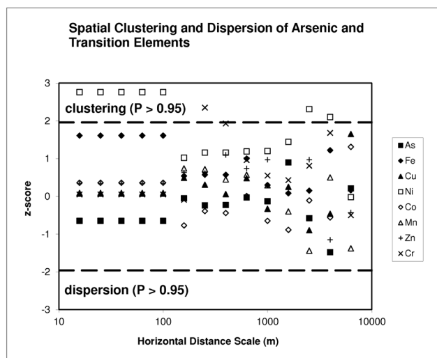
Fig. 6: Similar concentrations of Ni are clustered at horizontal distance scales 2500–4000 m and 10–100 m, while similar concentrations of Cr are clustered at a horizontal distance scale of 250 m. No other elements, including As, show clustering at any horizontal distance scale. The z-score is calculated using the Global Moran’s I-Test and the logarithms of concentrations (mg/L) in which values below the detection limit are set equal to the detection threshold (Mitchell 2005)
