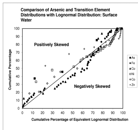
Fig. 3d: For each measured concentration of As, Fe, Cu, Ni, Co, and Zn in surface water, the percentage of measured concentrations less than or equal to that value is plotted against the percentage that would result from a lognormal distribution with the same mean and standard deviation as the set of logarithms of measured concentrations. Values below the detection limit are set equal to the detection threshold. All of the parameters follow a lognormal distribution with the exception of Zn, for which 40% of the measurements are below the detection limit.
