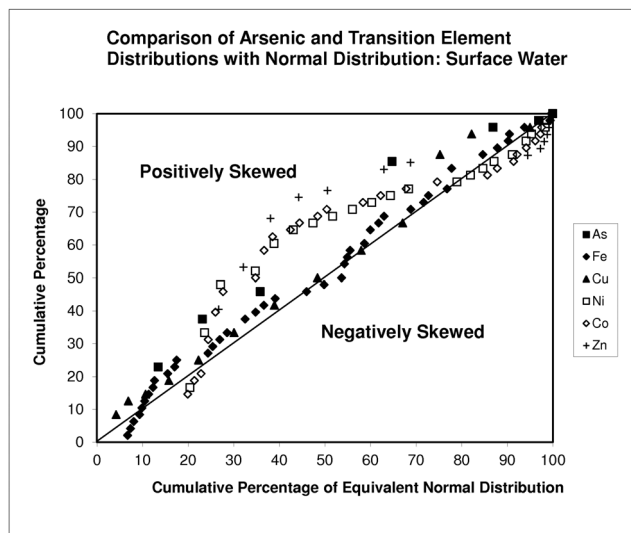
Fig. 3c: For each measured concentration of As, Fe, Cu, Ni, Co, and Zn in surface water, the percentage of measured concentrations less than or equal to that value is plotted against the percentage that would result from a normal distribution with the same mean and standard deviation as the set of measured concentrations. The parameters As, Fe, and Cu follow a normal distribution, but Ni, Co and Zn do not.
