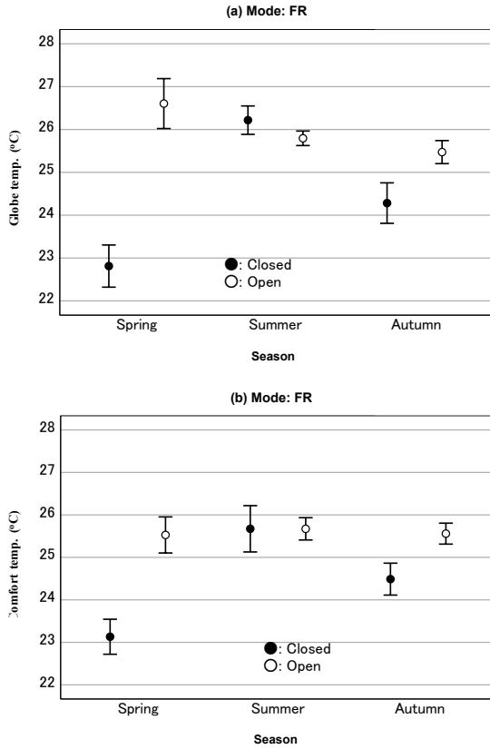
Figure 5: Seasonal variation of globe and comfort temperature for windows open and closed (at 95% confidence level).
