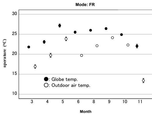
Figure 2: Month mean globe temperature and outdoor air temperature (at 95% confidence level).
