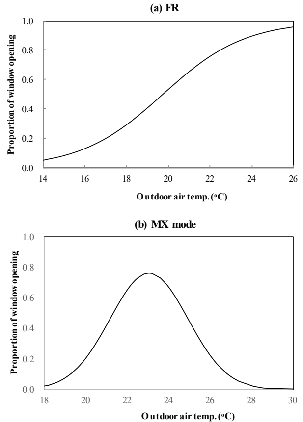
Figure 6: Relation between the window opening and outdoor air temperature.
