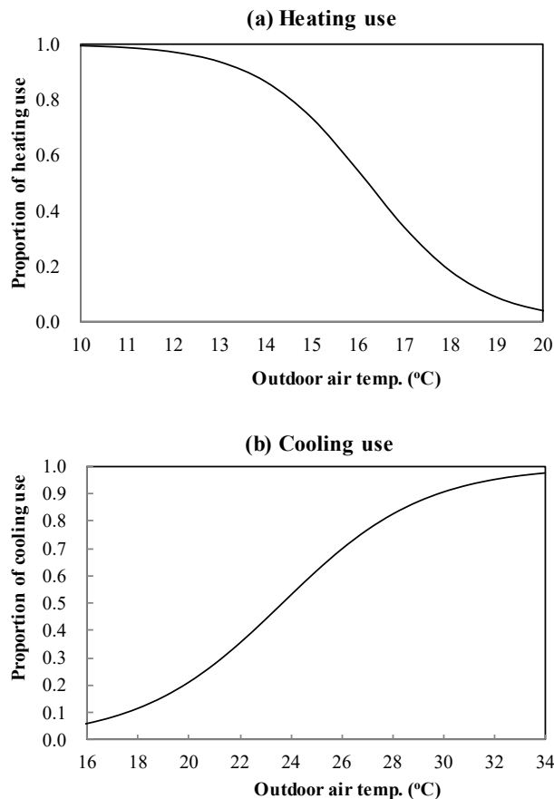
Figure 9: Relation between the heating use or cooling use and outdoor air temperature.
