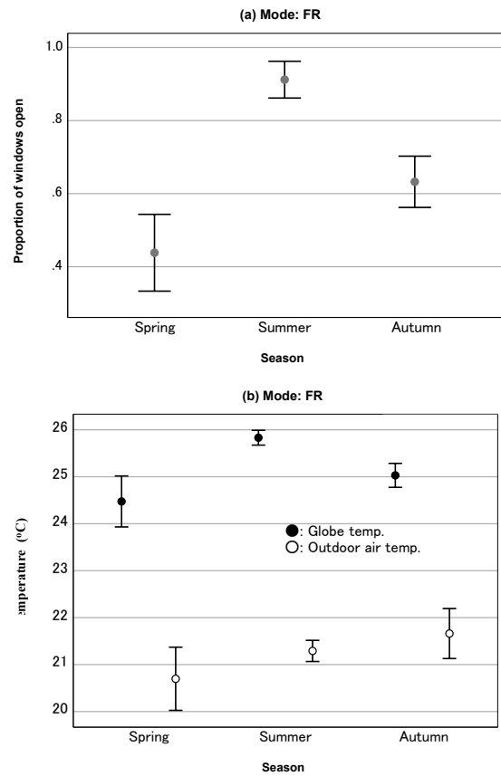
Figure 3: The proportion of open windows, globe temperature and outdoor air temperature in each season (at 95% confidence level).
