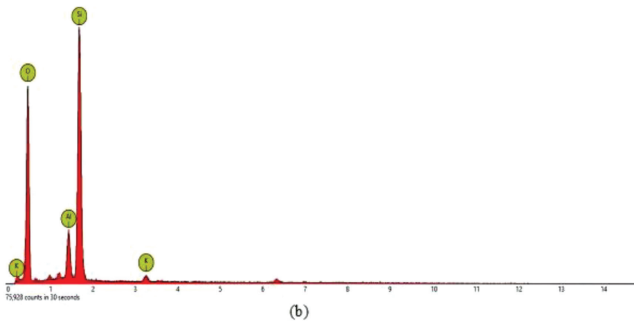
Fig. 5: (a) SEM micrograph and (b) EDS spectrograph of 40 wt. % SP reinforced carbon composite with the elemental composition
