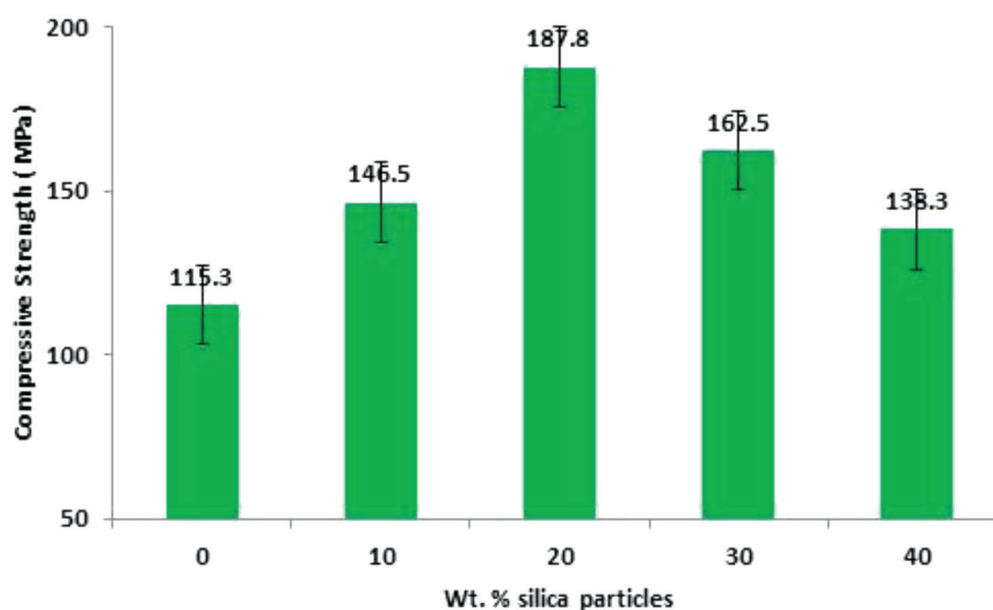
Fig. 6: Variation of compressive strength with silica particles addition
