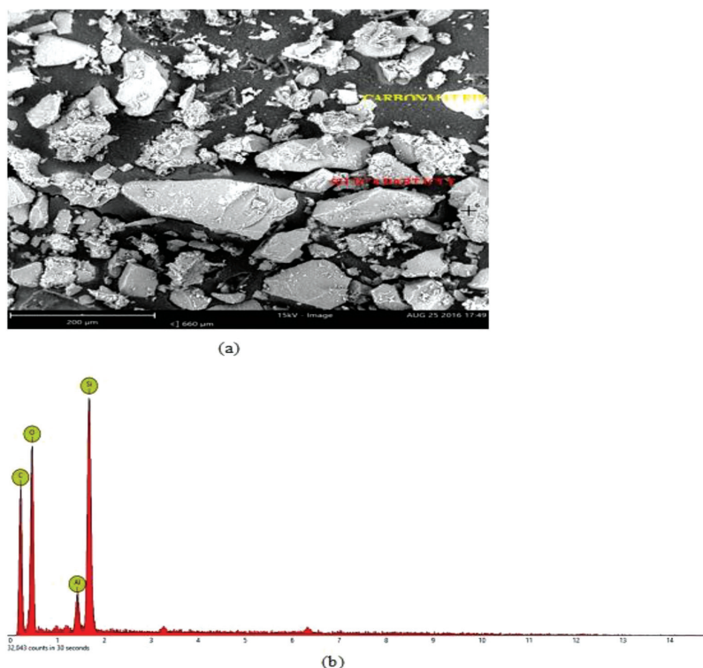
Fig. 4: (a) SEM micrograph and (b) EDS spectrograph of 20 wt. % SP reinforced carbon composite with the elemental composition
