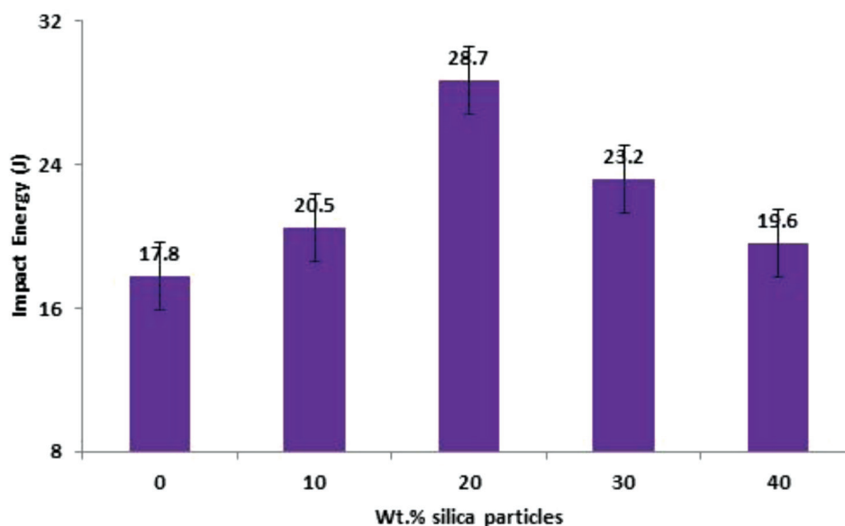
Fig. 8: Variation of impact energy with silica particles addition
