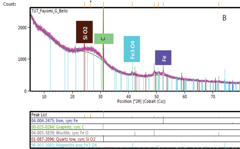
Fig. 2: XRD image of coconut shells [3]
