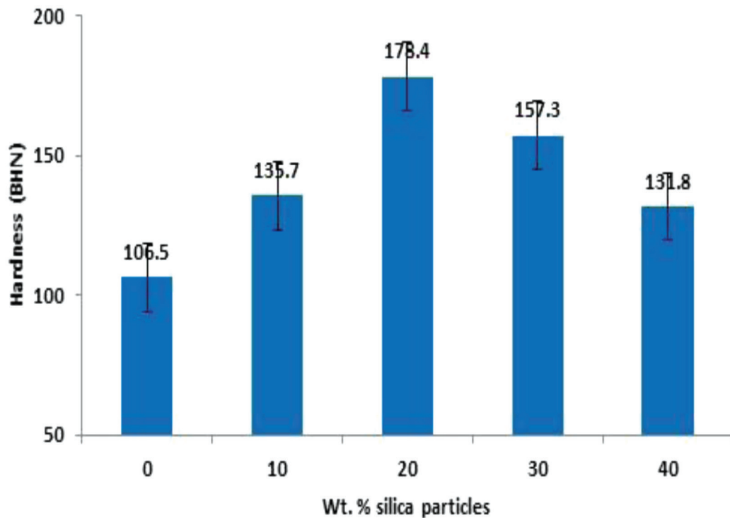
Fig. 7: Variation of hardness with silica particles addition
