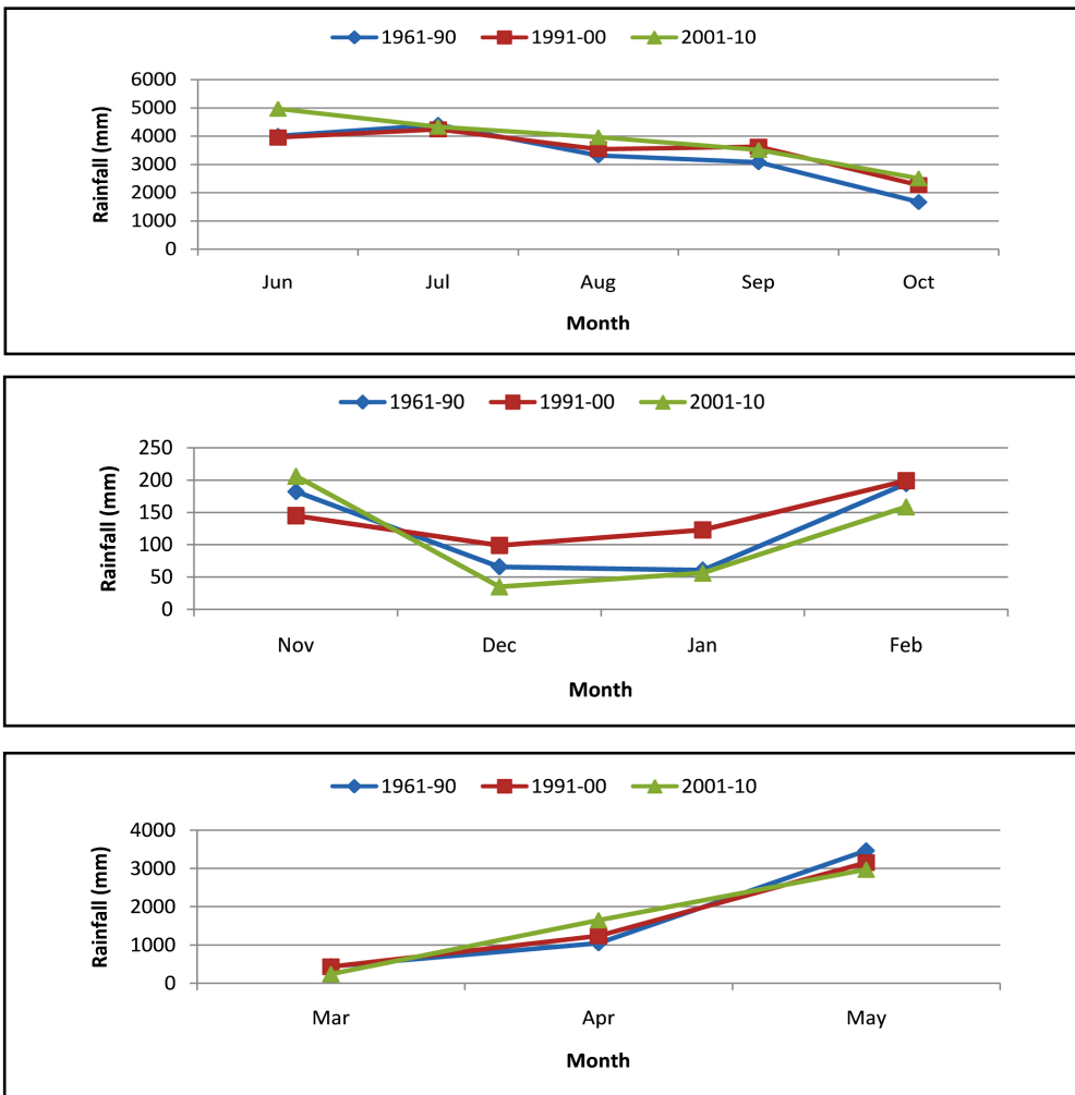
Fig 5 : Seasonal variations of rainfall in the study area over time
