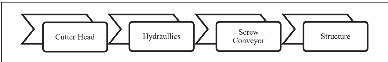
Figure 2: Reliability block diagram of EPBTBM
