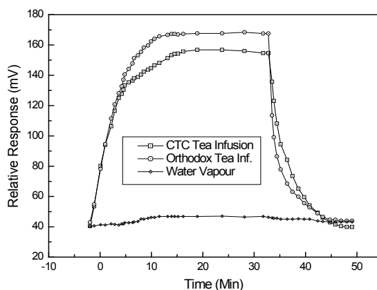
Fig.4: Response of the ZnO nanowire gas sensors measured at temperature 200°C with Orthodox tea and CTC tea infusion (at 100°C) and compared with response in plain water vapour.
