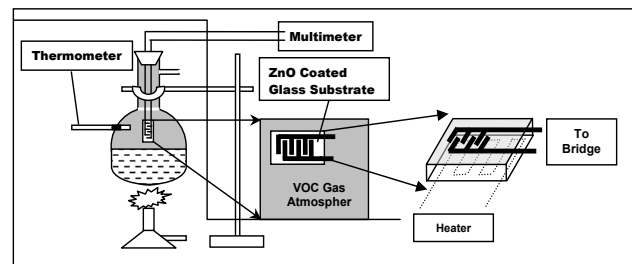
Fig.2: Schematic picture of sample measurement system in static gas environment
